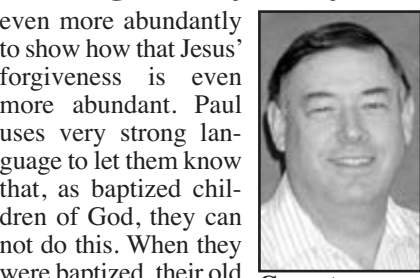
Compton
